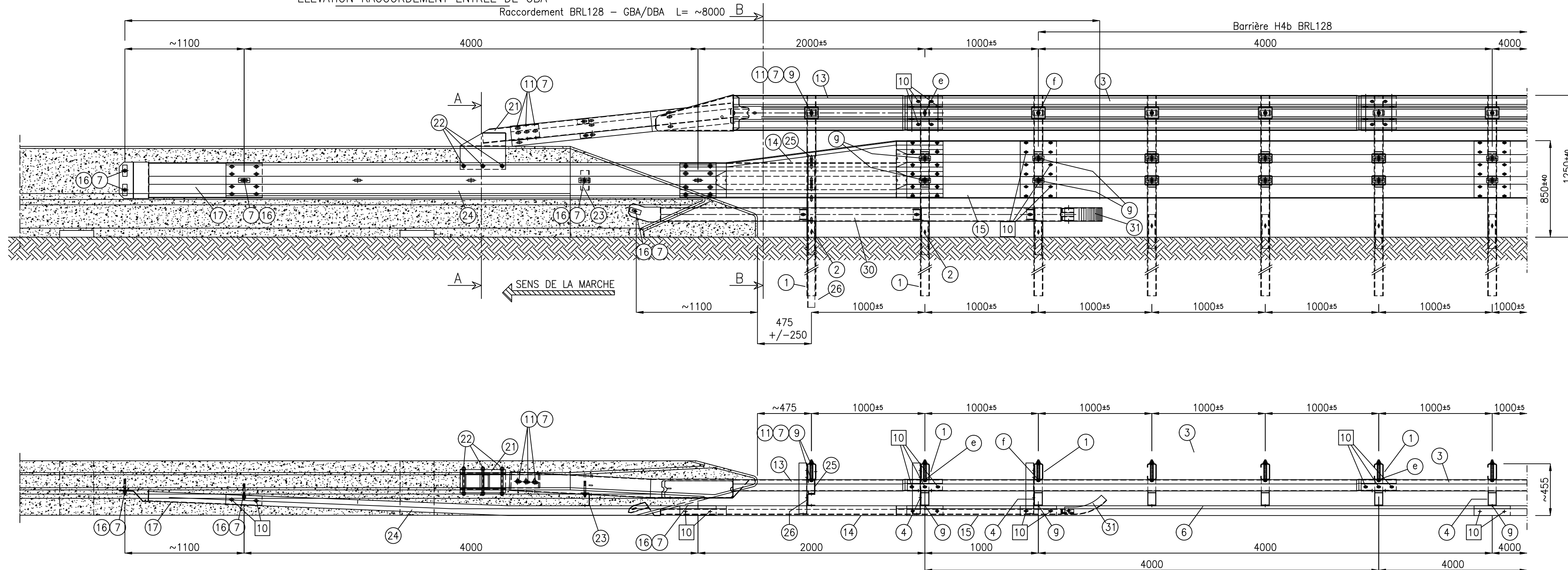
ELEVATION RACCORDEMENT ENTREE DE GBA
